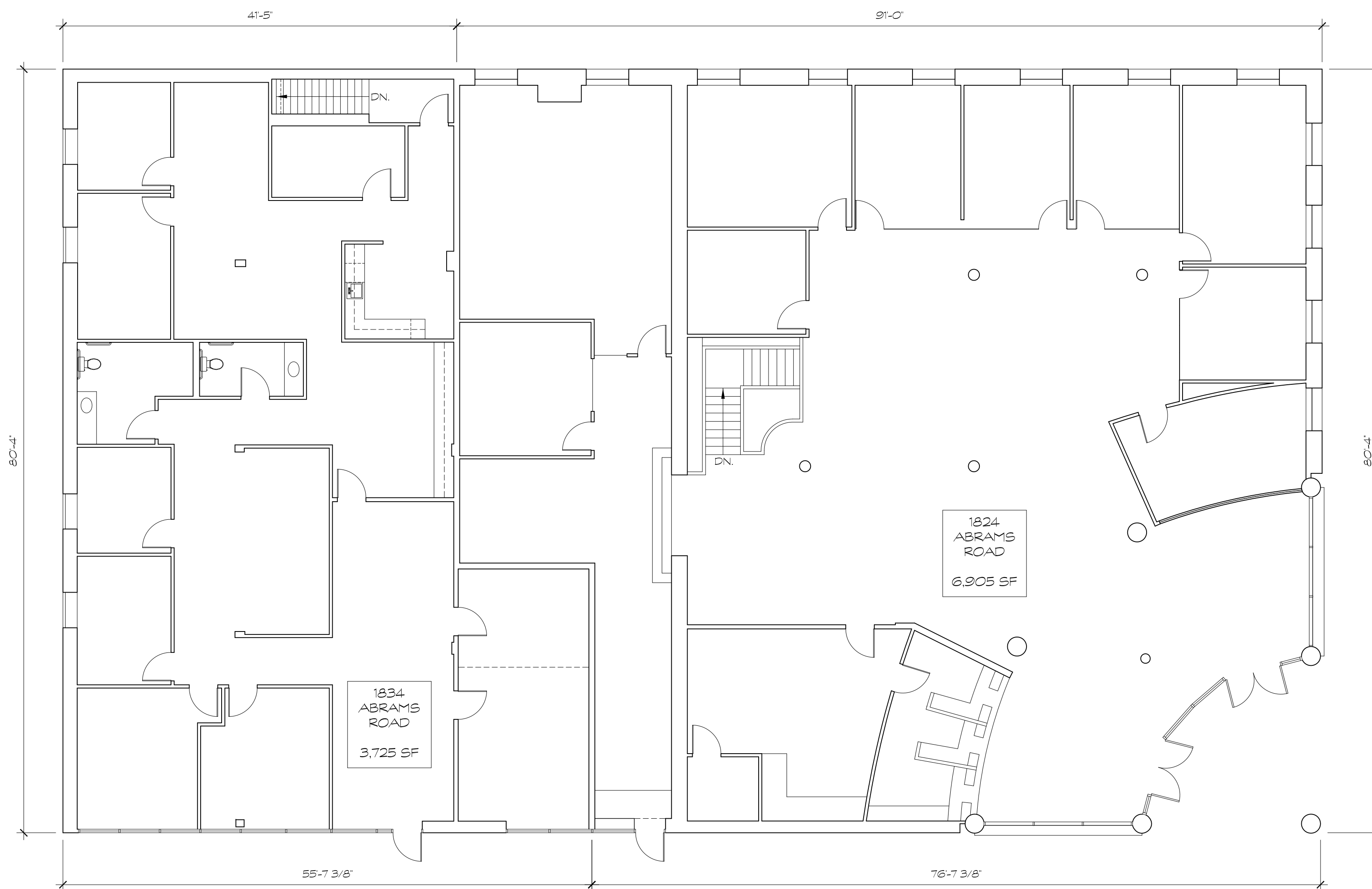
FIRST FLOOR LEASE OUTLINE DRAWING 454-11-03 First Floor Lease Outline Drawing 01-01
